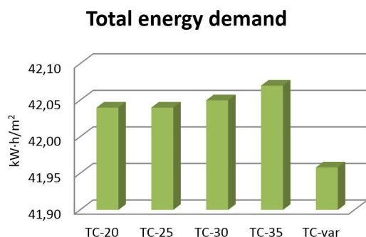
Figure 8. Building model 15 % Windows North façade. Total energy demand.
