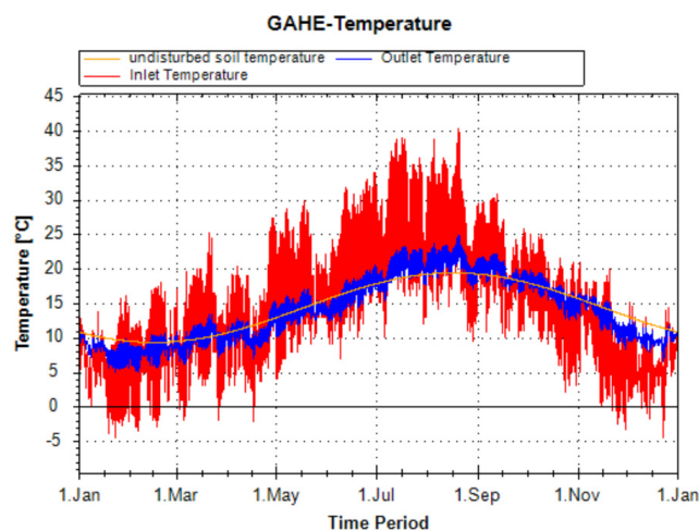
Figure 5. Dynamic simulation for fresh air intake temperatures through the GSHX.
