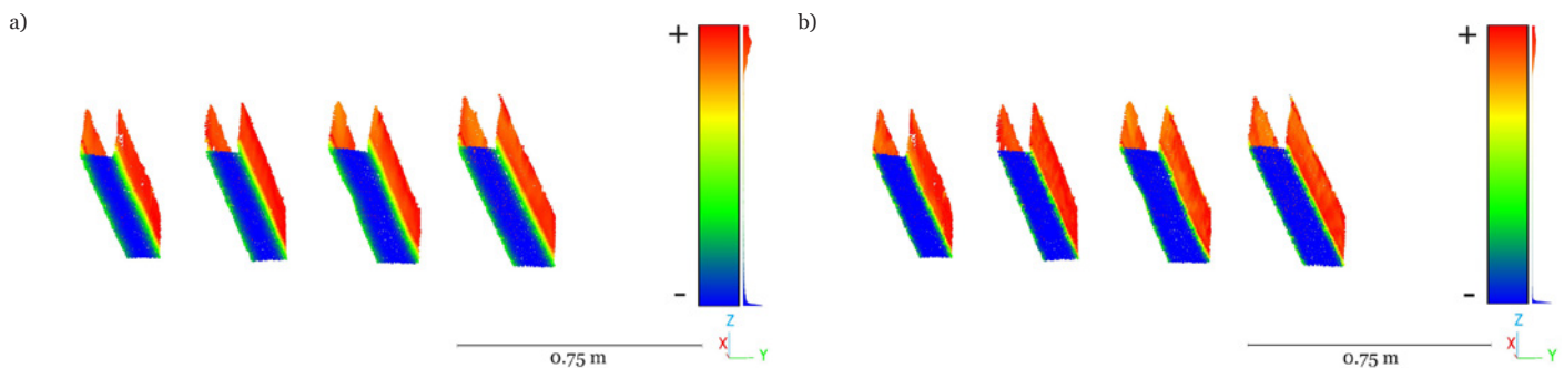
Figure 16. 3D point cloud of the best parameters for the Random Forest: a) Verticality (0.025), b) Verticality (0.05).
