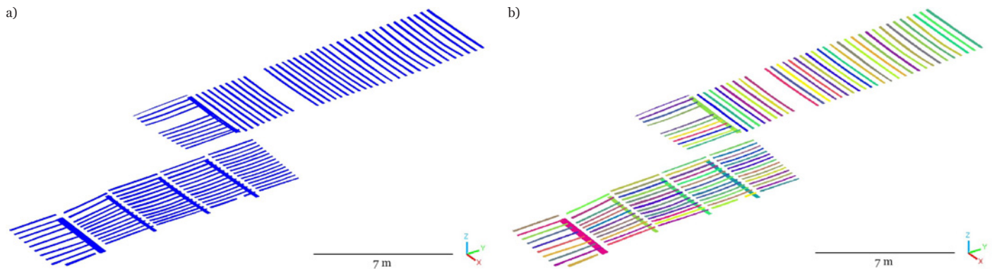
Figure 18. Results after applying the first step: a) original input; b) element clusterization by using the connected components algorithm.
