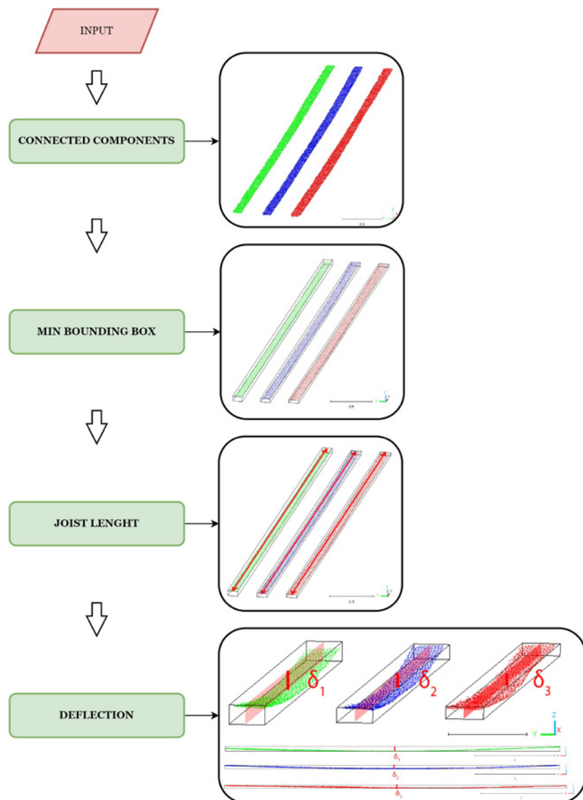
Figure 9. Scheme of the proposed deflection analysis.
