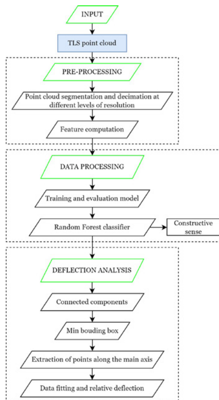
Figure 3. Scheme of the proposed workflow.
