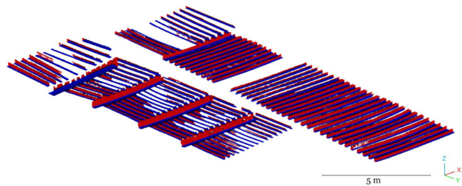
Figure 6. 3D point cloud segmented on third level of classification. The red represents the class joist faces and the blue the class joist edges. This classification is carried out manually by the operator with the aim of evaluating the algorithm’s behaviour.
