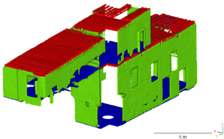
Figure 11. 3D point cloud of the prediction on first level of classification. The red points represent the slab class. The blue points the class floor and the green the class vertical walls.
