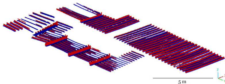
Figure 13. 3D point cloud of the prediction on third level of classification. The red points represent the joist face class. The blue points represent the joist edge class.
