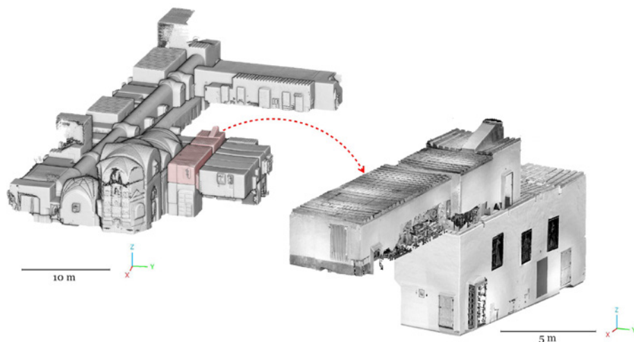
Figure 1. 3D point cloud of the convent Nuestra Señora de Gracia. The red zone highlights the area of interest for this study Adapted from Villanueva-Llauradó et al. 2022 [9] and Sánchez-Aparicio et al. 2023 [10].
