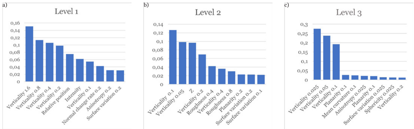
Figure 15. Feature importance results: a) Level 1, b) Level 2 and c) Level 3.
