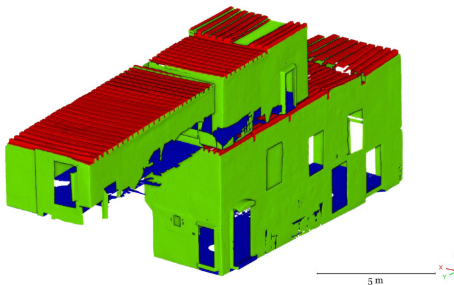
Figure 4. 3D point cloud segmented on first level of classification. The red color represents the class slabs. The blue color represents the class floors and the green represent the class vertical walls. This classification is carried out manually by the operator with the aim of evaluating the algorithm's behaviour.
