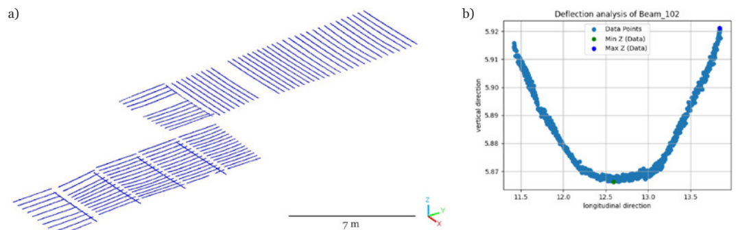
Figure 19. Results after applying the second step: a) extraction of the beam axis by using the Minimum Bounding Rectangle algorithm; b) example of the graph obtained in the beam number 102 (units expressed in metres).
