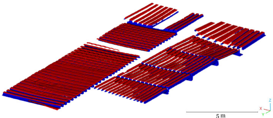
Figure 5. 3D point cloud segmented on second level of classification. The red color represents the class timber boards and the blue the timber joists. This classification is carried out manually by the operator with the aim of evaluating the algorithm's behaviour.
