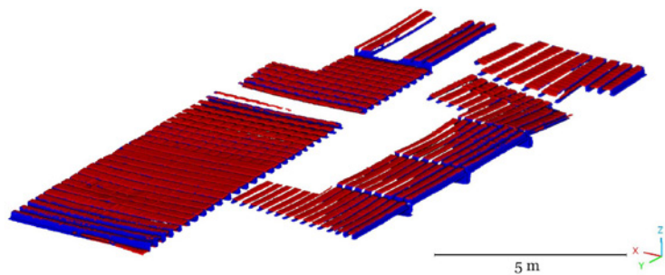
Figure 12. 3D point cloud of the prediction on second level of classification. The red points represent the class timber boards. The blue points represent the class timber joists.
