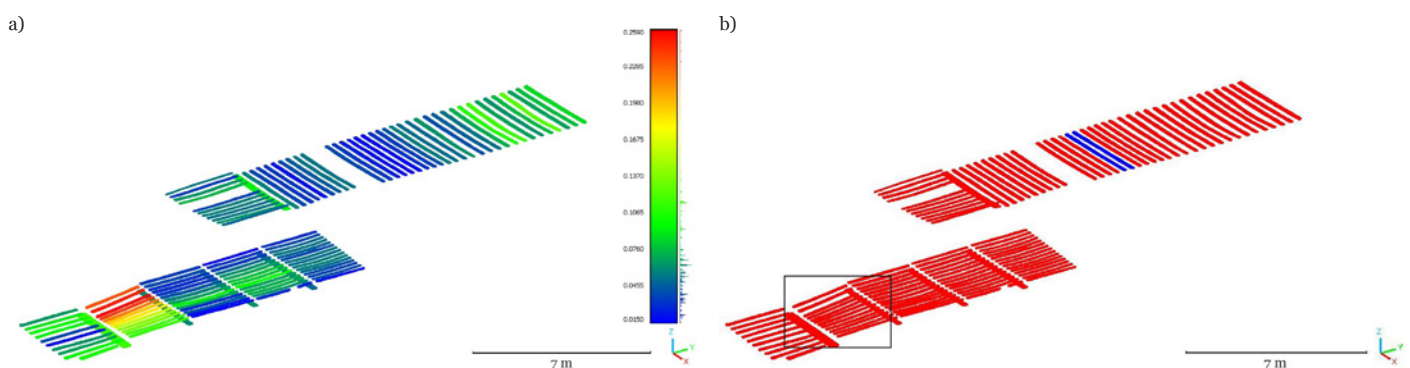
Figure 20. Results of the final 3D point cloud: a) with the maximum deflection layer (difference between the highest and the lowest point); b) with a layer that represents in blue the beams which meet the relative deflection ( L/300 ) threshold and in red those that don't fulfil this requirement (joists within the square was not properly calculated due to the impossibility of horizontal alignment).
